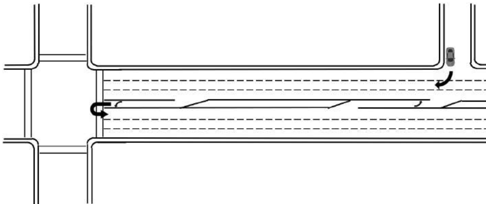
Exhibit 6-4 Access Management with Downstream U-turns
