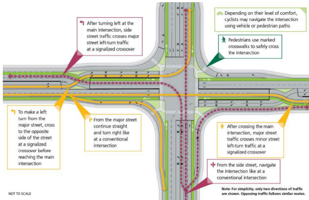
Exhibit 6-12 Displaced Left-Turn Intersection Layout
