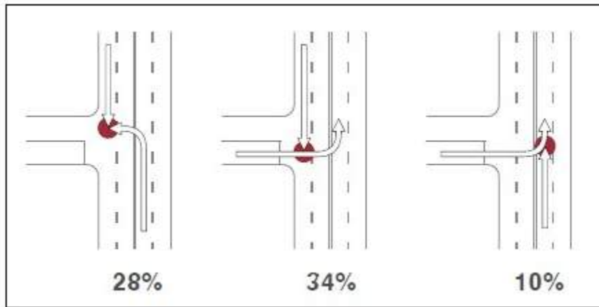
Exhibit 6-3 Driveway Collision Types
