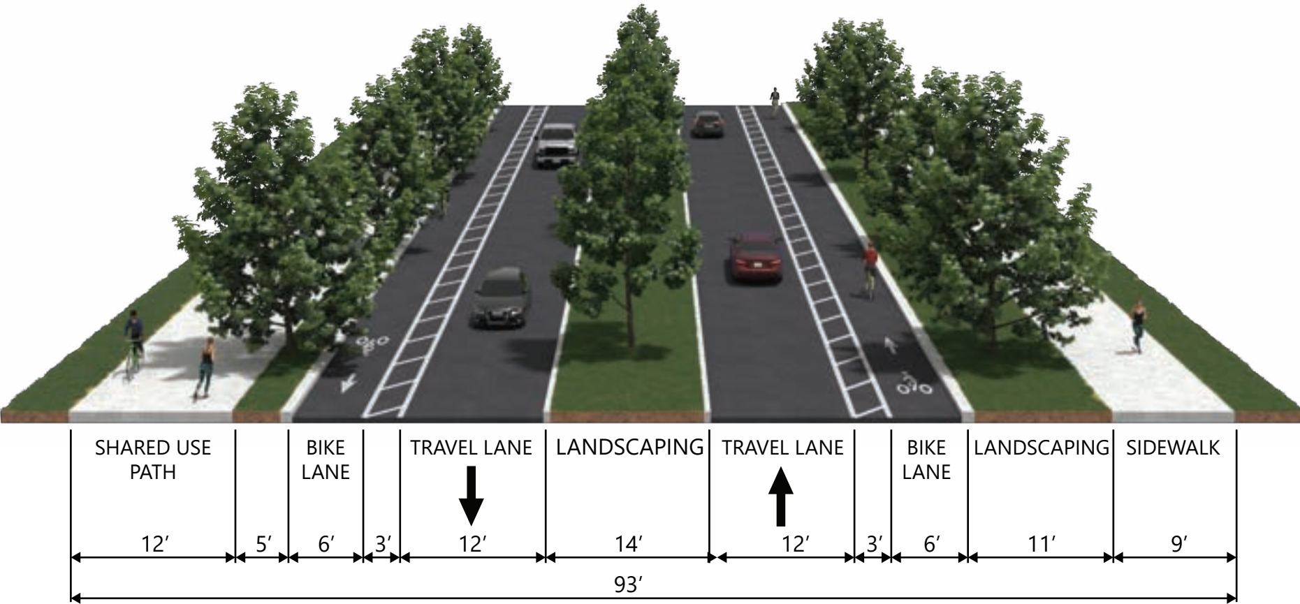
ALTERNATIVE 4: BUFFERED BIKE LANES AND WIDENED SHARED USE PATH
