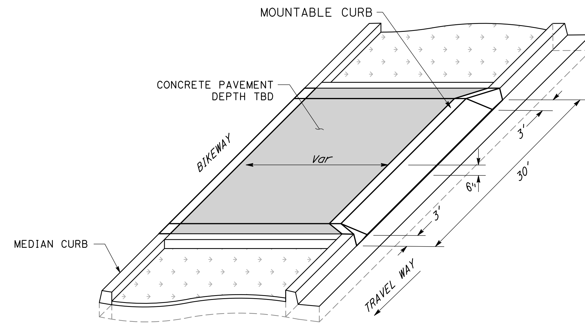
MAINTENANCE VEHICLE PULLOUT NO SCALE
