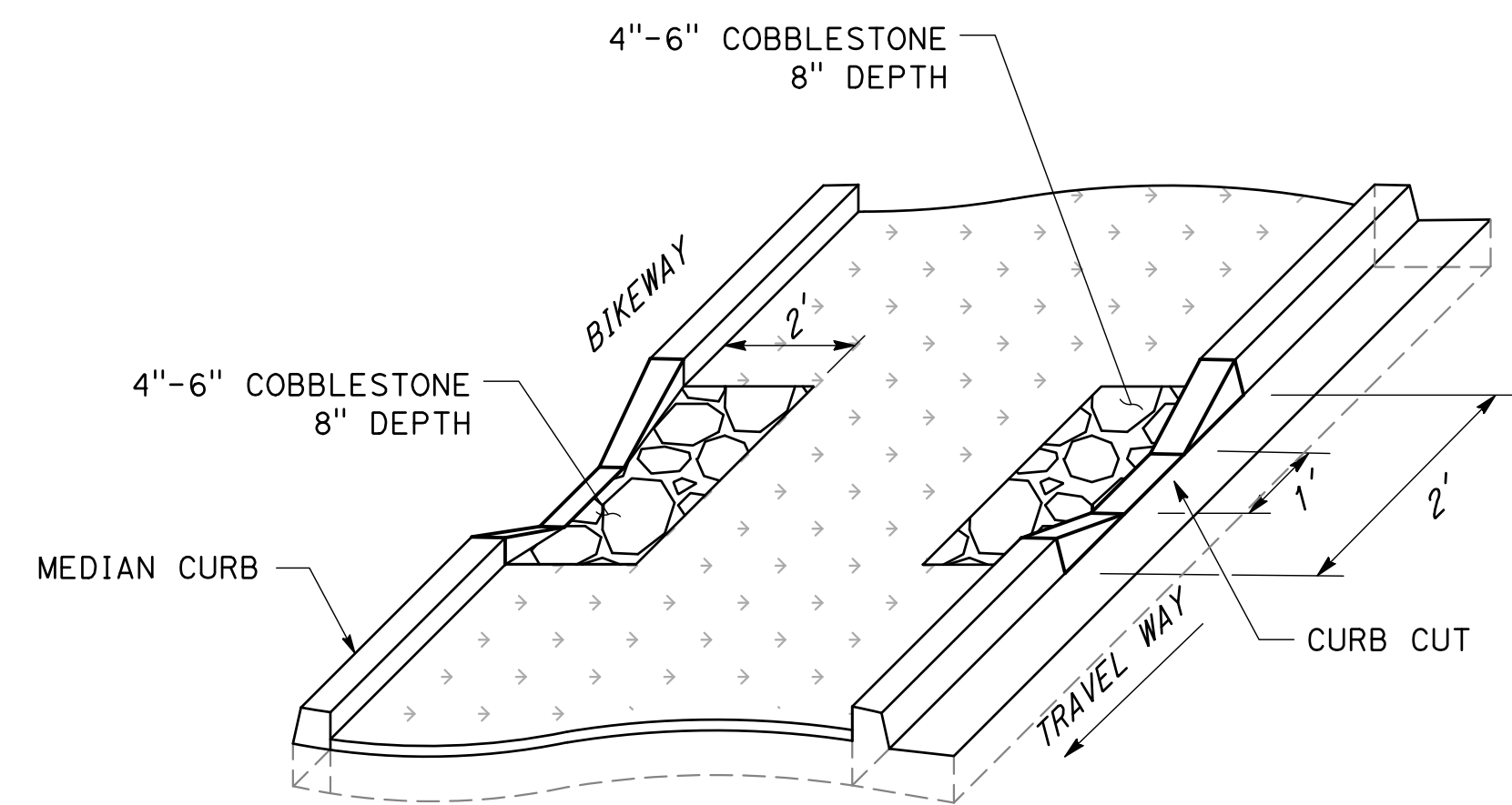
PLANTER MEDIAN CURB CUT AND COBBLESTONE DETAIL NO SCALE
